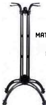
TT 106 EXT CA UMBRELLA BASE MATERIAL: CAST ALUMINUM HEIGHT: 28.5" SPIDER LENGTH: 27" BASE SPREAD: 34" WEIGHT: 25LBS
